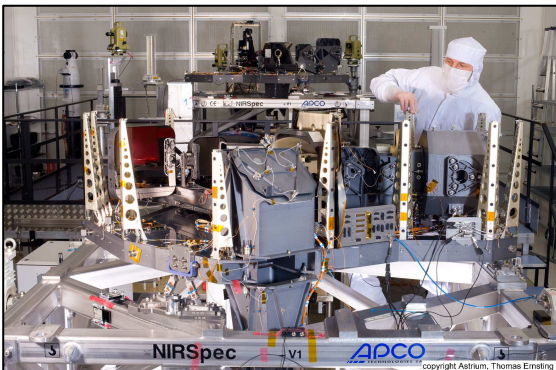
NIRSpec Instrument
